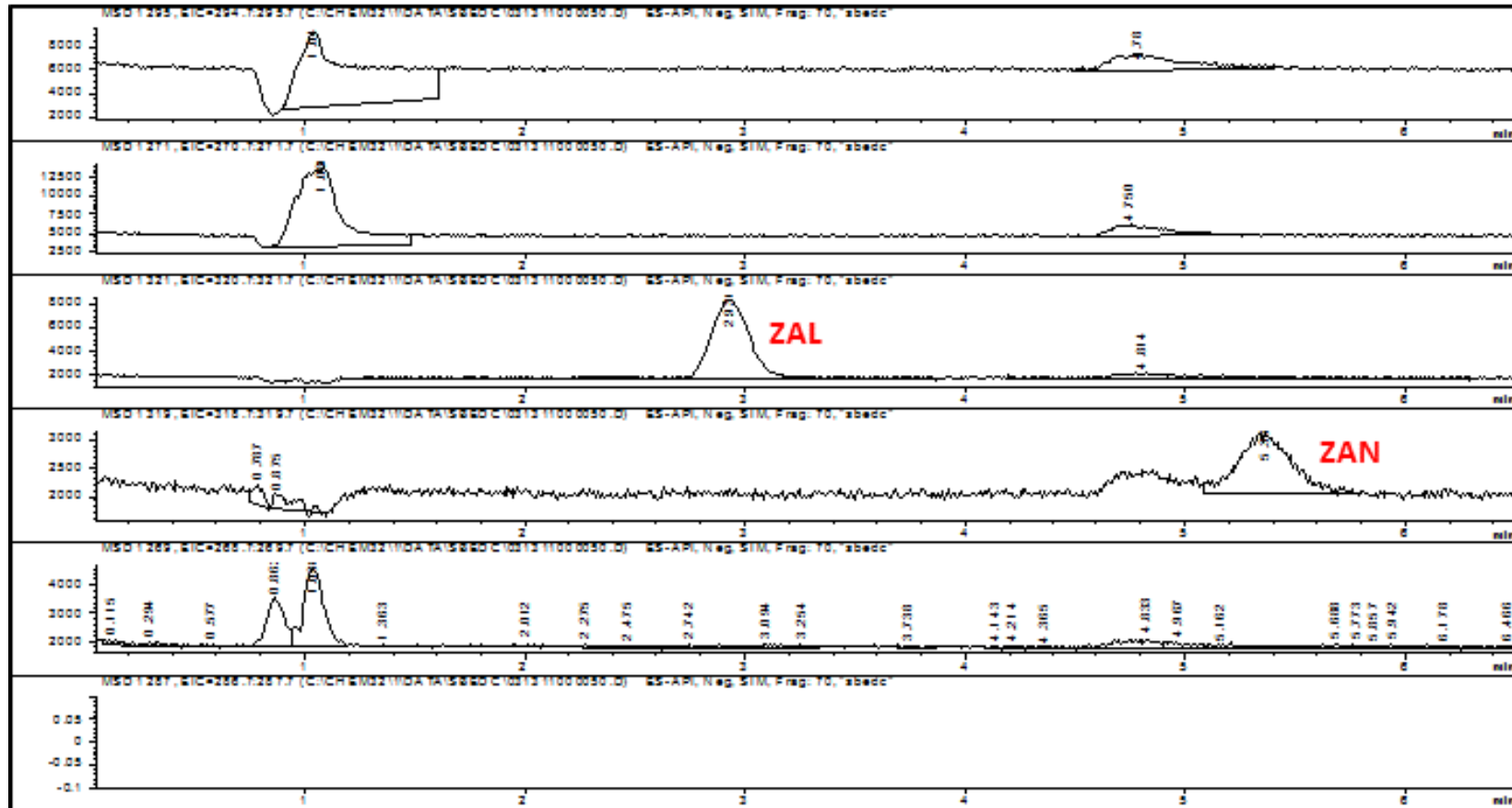
Figure A-19 Example chromatogram from the aqueous solution of the ZAL only dead plant exposure on day 14 of the softstem bulrush experiment. The X-axis represents the retention time and the Y-axis represents the peak heights with the target compound names listed in red on the right side of the associated peaks.
